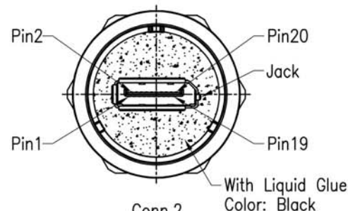
Conn.2
