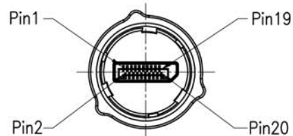
Conn.1 Pin Assignments Front View
