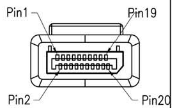
Conn.2 Pin Assignments Front View
