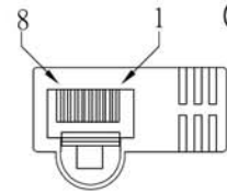
View of Mating Face of Connector
