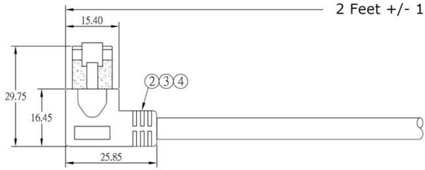
RJ45 Male (Unshielded)
