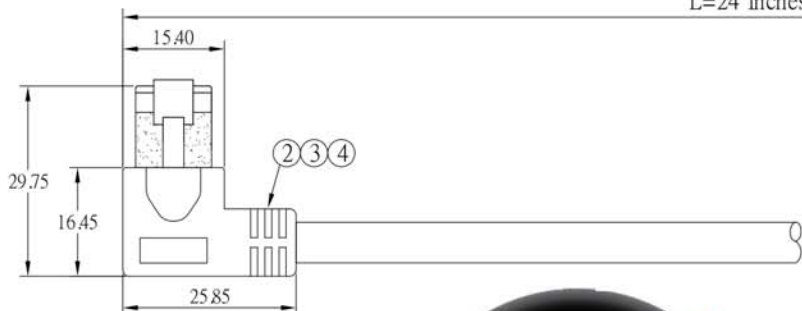
RJ45 Male (Shielded)
