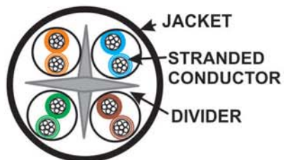
Cross Section View
