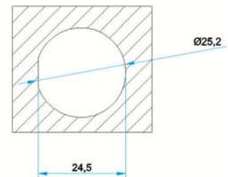
Installation hole figure
