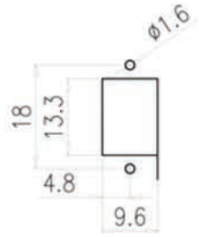
SUGGESTED PANEL CUTOUT
