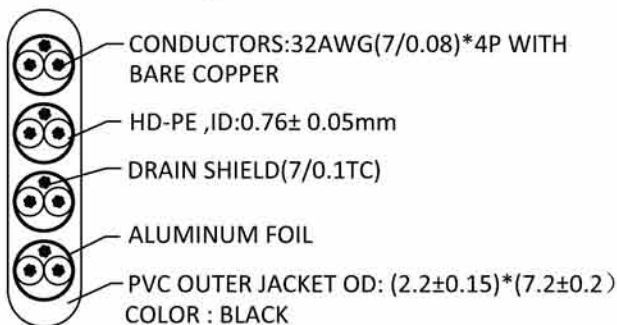
CORD SPECIFICATION
