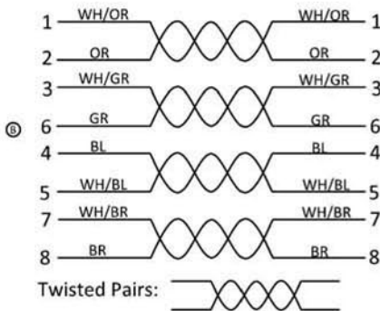
J1 SIDE TIA/EIA-568-B.2 PIN ASSIGNMENT J2 SIDE
