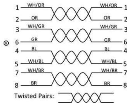
J1 SIDE TIA/EIA-568-B.2 PIN ASSIGNMENT J2 SIDE
