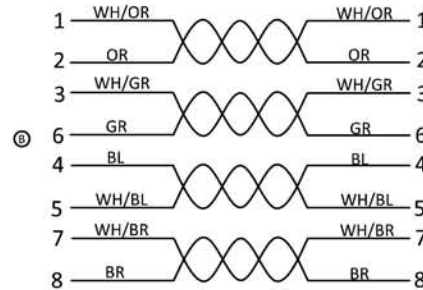
J1 SIDE TIA/EIA-568-B.2 PIN ASSIGNMENT J2 SIDE
