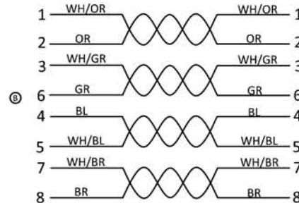
J1 SIDE TIA/EIA-568-B.2 PIN ASSIGNMENT J2 SIDE
