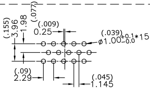
15 Pin Female Connector PCB Pin Layout Scale 2:1
